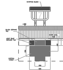
2 TARGET DETAIL SCALE 1:30
