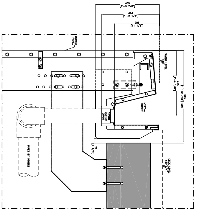
2 TOP 3' POOL GUTTER DRAIN SCALE 1/8"=1'-0"
